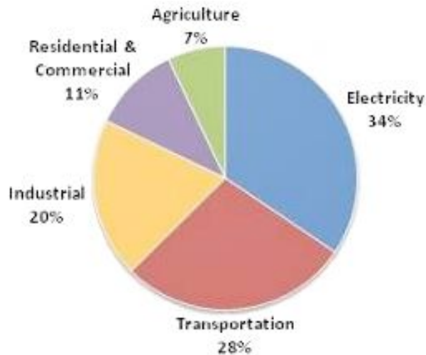
Figure 1 U.S. greenhouse gas emissions by economic sector (2007)
